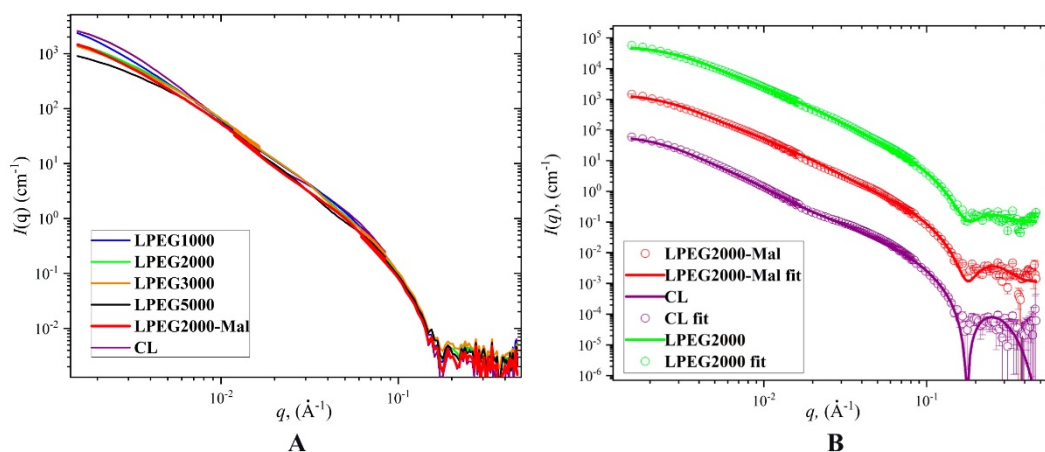
Figure 3. SANS scattering curves. The experimental (a) and the selected (b) SANS data with their fits. Please note, that the scattering curves are vertically shifted for clarity in Figure 3B.
